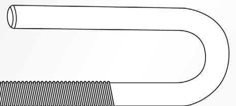
Item No. 2 Top Strap Through Post 300mm x 16mm
